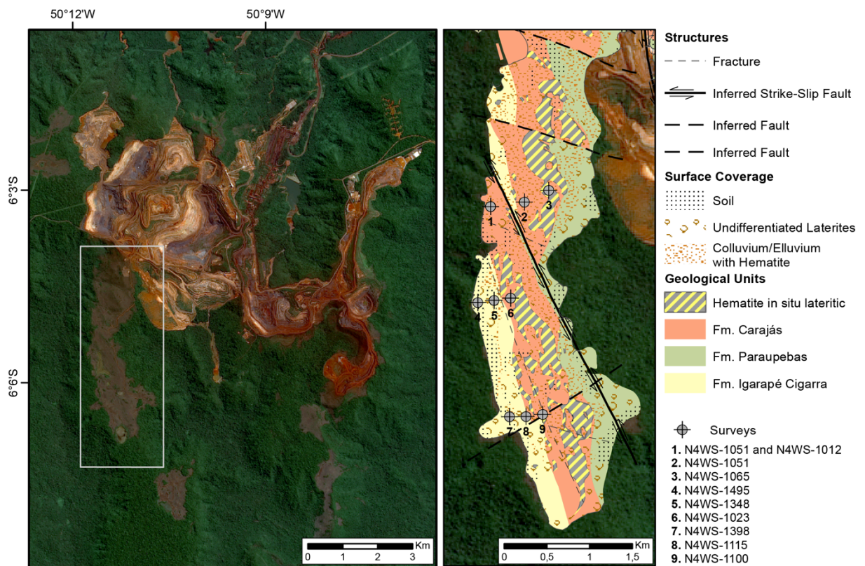
Figure 4.2 Landsat 8 Operational Land Imager (OLI) sensor satellite image on the left showing the open pit of the N4 mine; the N4WS body is highlighted. On the right is the geological map of the N4WS body, focusing on the lithotypes described in the Serra Norte plateaus (Tolbert et al., 1971; Resende and Barbosa, 1972; Macambira, 2003). The studied drill holes are shown on the map and indicate the direction of the section.
